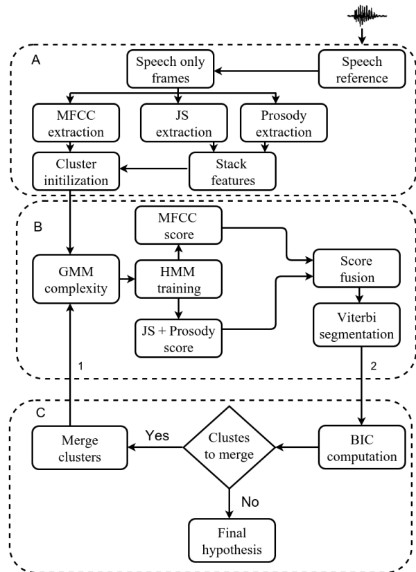
Figure 1: Baseline speaker diarization architecture which draws a classical bottom-up agglomerative approach based on HMM/GMM modeling. The clustering technique is driven by Bayesian Information Criterion.
