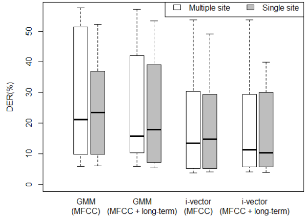
Figure 4: Box plots of single- (grey) and multiple-site (white) scenario test recordings. Four different combinations are reported, resulting from the mixing of clustering approaches and feature sets.
