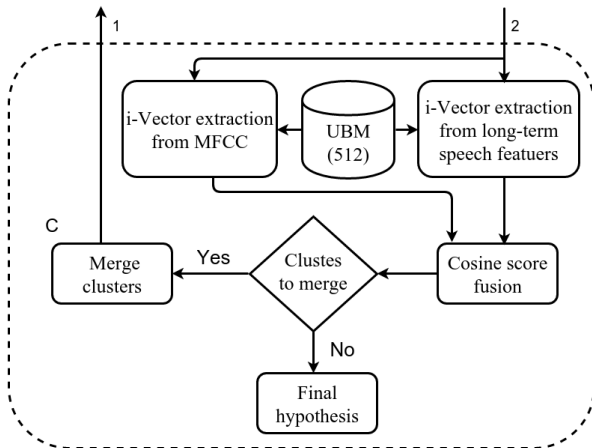
Figure 2: Proposed i -vector based speaker clustering architecture based on a weighted cosine-distance among i -vectors.
